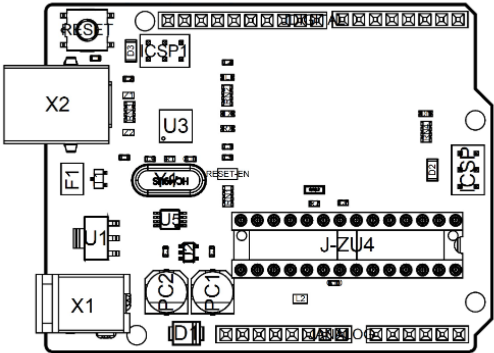
Board topology
